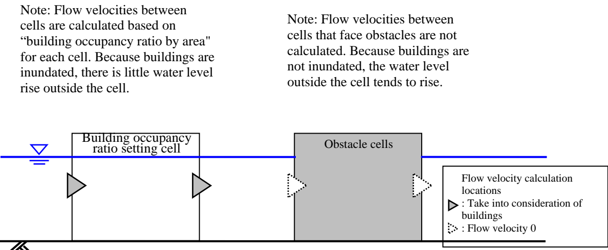
Figure III—8 Schematic of building resistance (left) and obstacle resistance (right) (side view)
