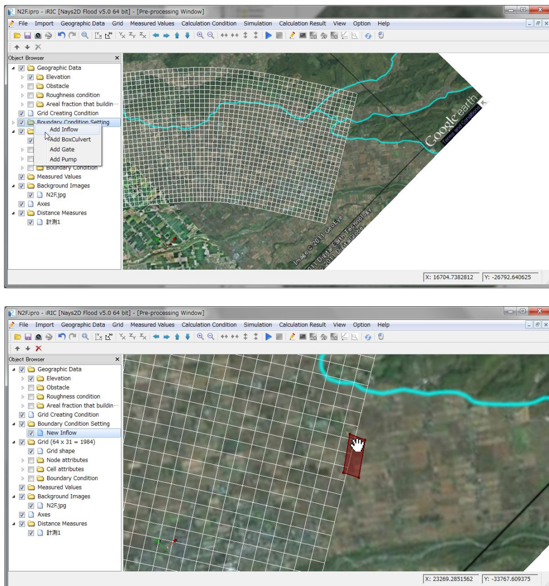
Figure III-6 Dialog for setting [River Inflow]
