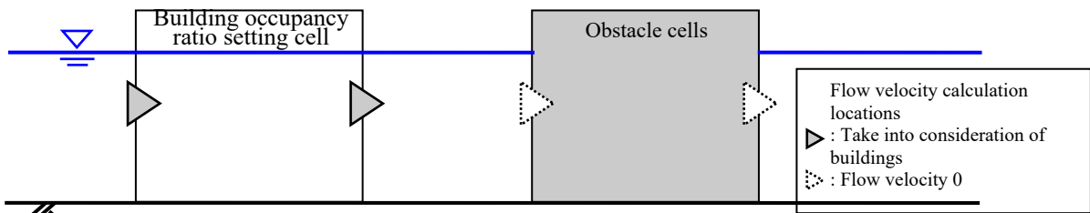
Figure III—8 Schematic of building resistance (left) and obstacle resistance (right) (side view)
