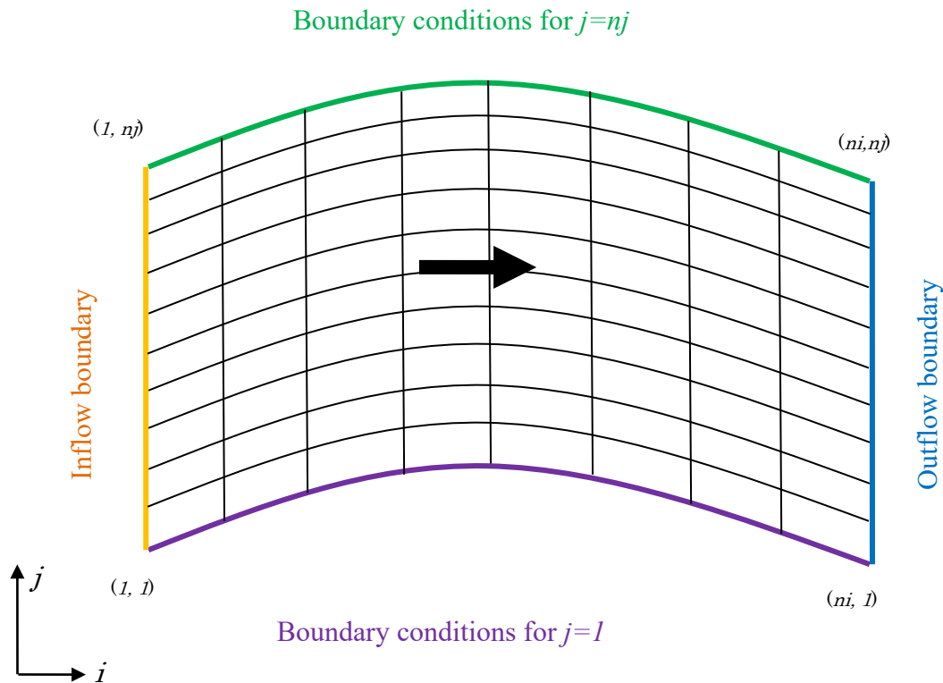
Figure III-1 Grid cell modeling
