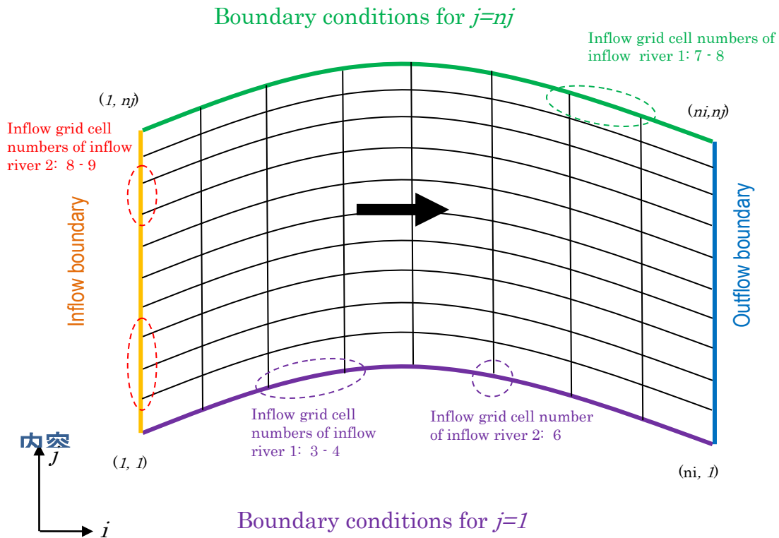
Figure IV-2 Input file for grid cell numbers of inflow
