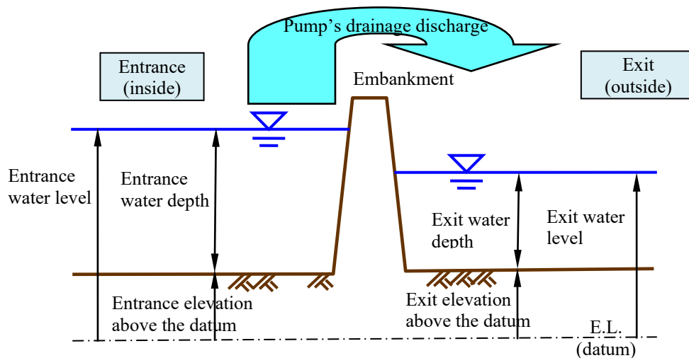
Figure II—3 Schematic of a pump (side view)
