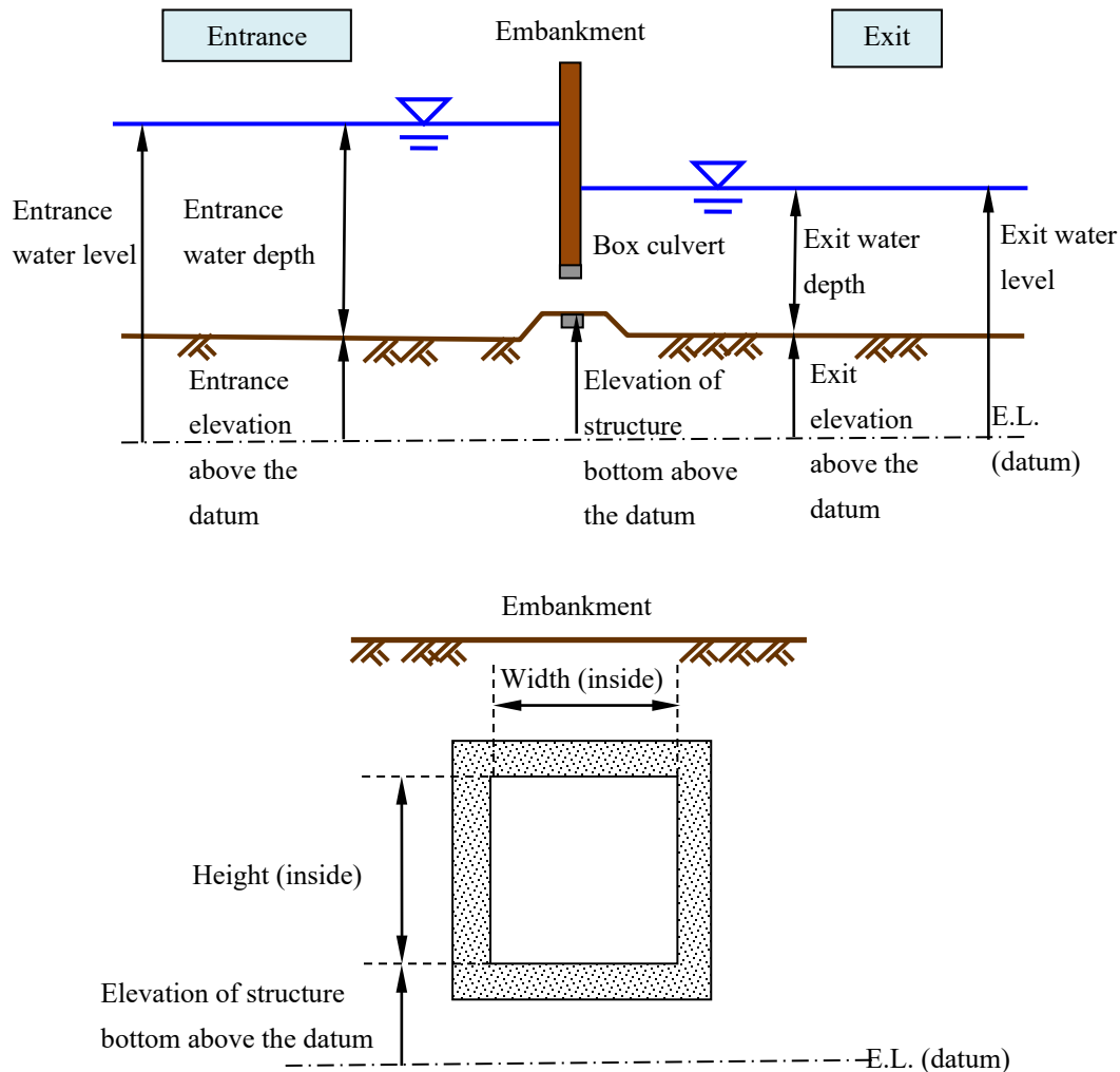
Figure II—1 Schematic of a box culvert (side view and section view)
