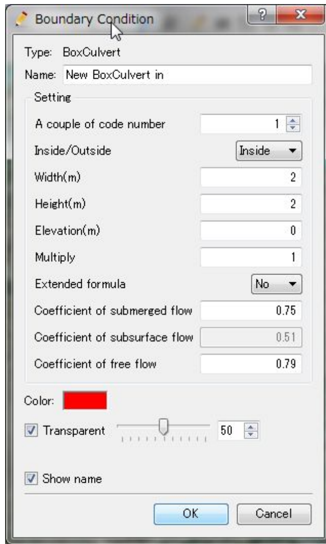
Figure III – 10 Boundary conditions setting window
