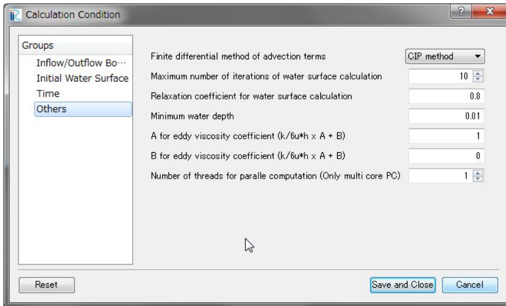
Figure III-5 Dialog for setting [Other information]
