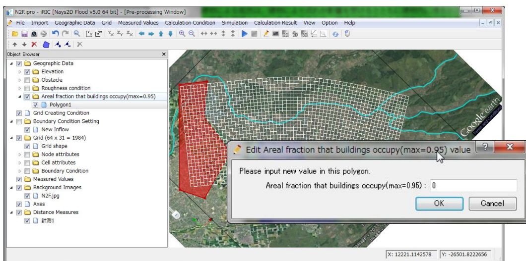
Figure III—7 Windows to set “Areal fraction that building occupy” or building occupancy ratio by area
