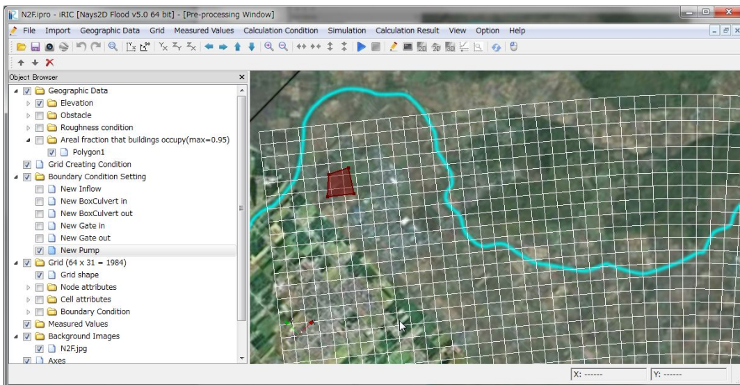
Figure III– 13 Pump setting window
