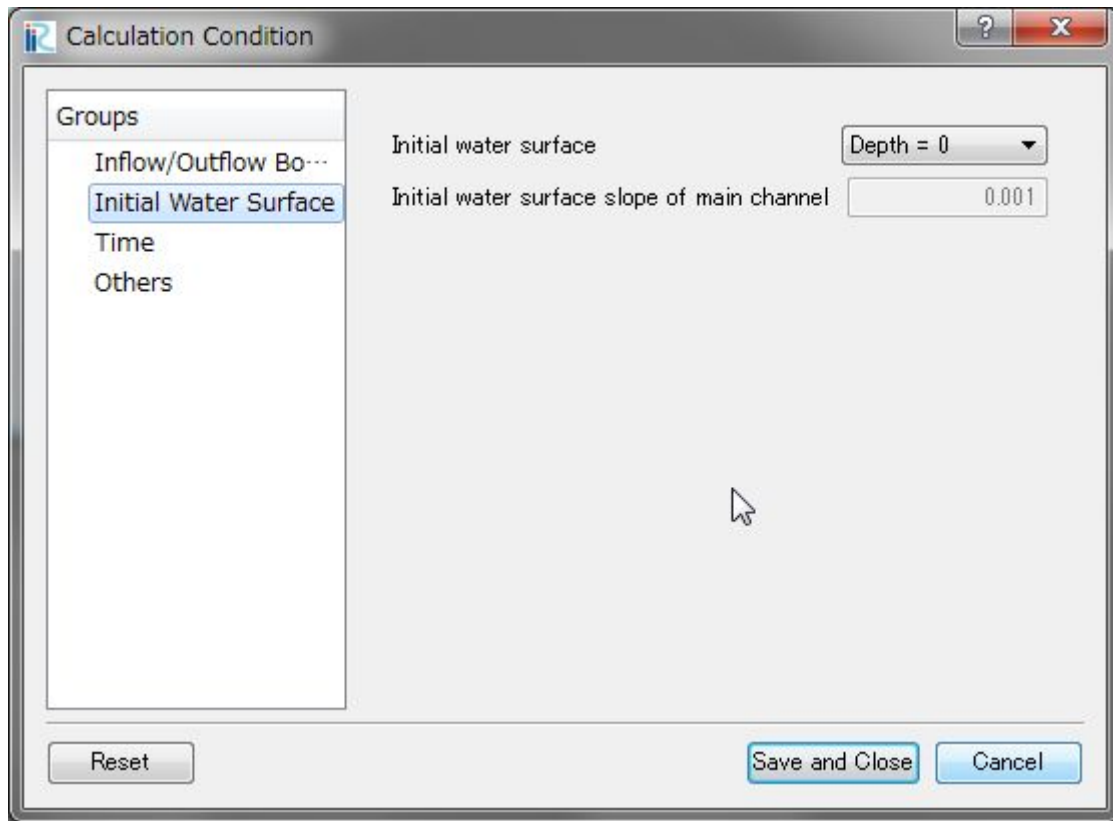
Figure III-3 Dialog for setting [Initial water surface]
