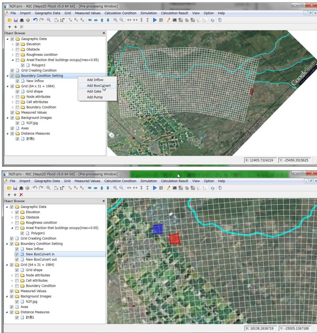
Figure III—9 Box culvert setting window
