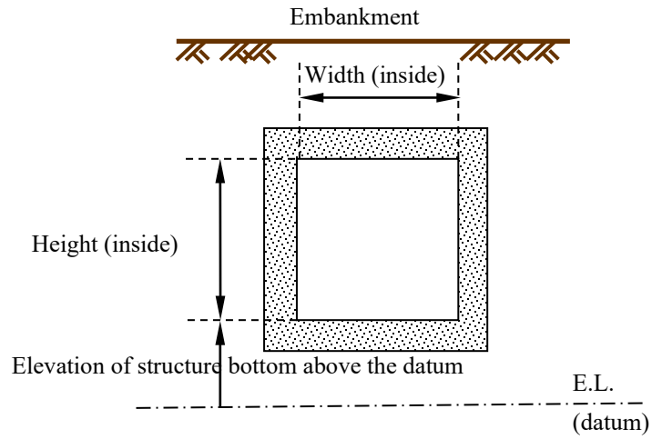
Figure II—2 Schematic of a sluice pipe (side view and section view)
